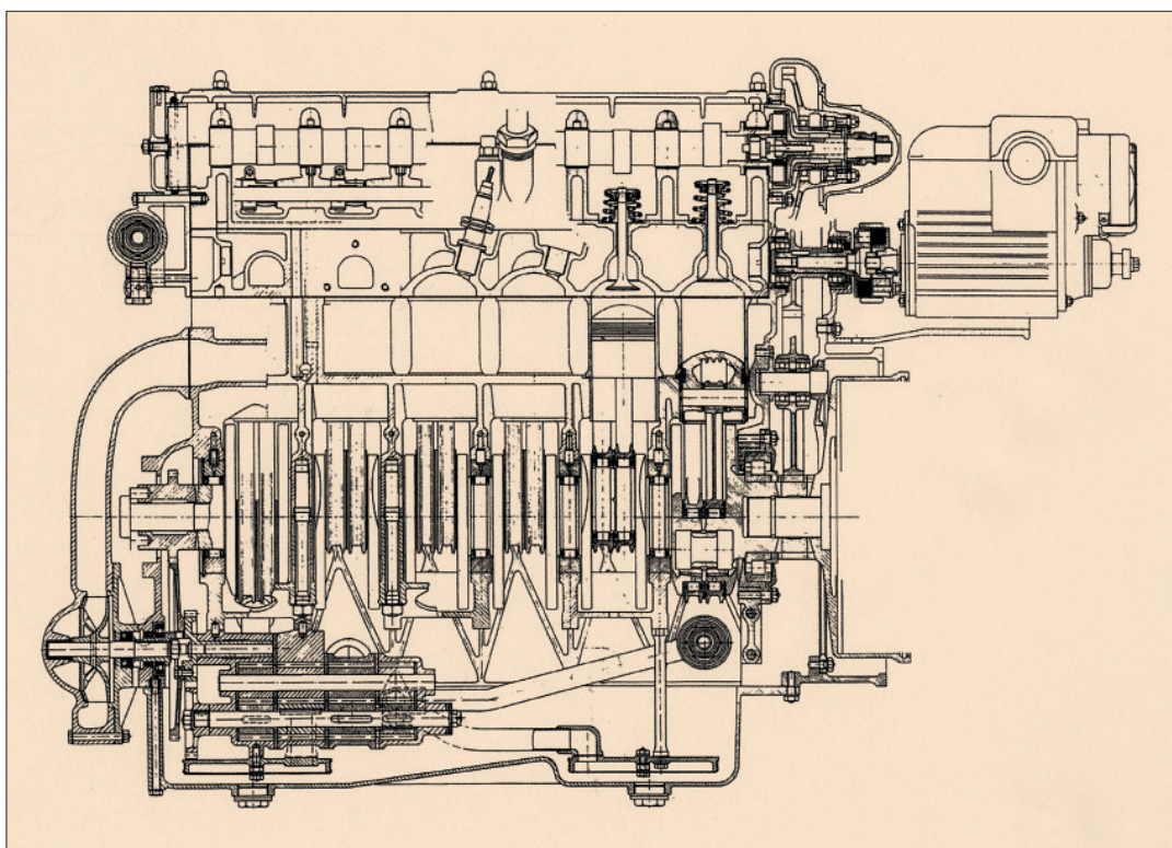
LEFT This view of the Type 537 V-12 planned by Auto Union for its E-Type in 1940 showed gear-type cam and blower drives at its flywheel end near an extra-large roller bearing
