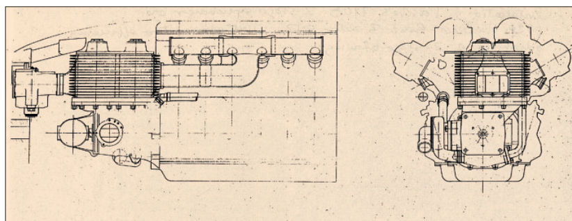
ABOVE & LEFT Porsche's experimental Type 108 twin-blower array for Mercedes-Benz had rotors of equal length and differing diameter. Its design fitted to the front of the M154 twelve
