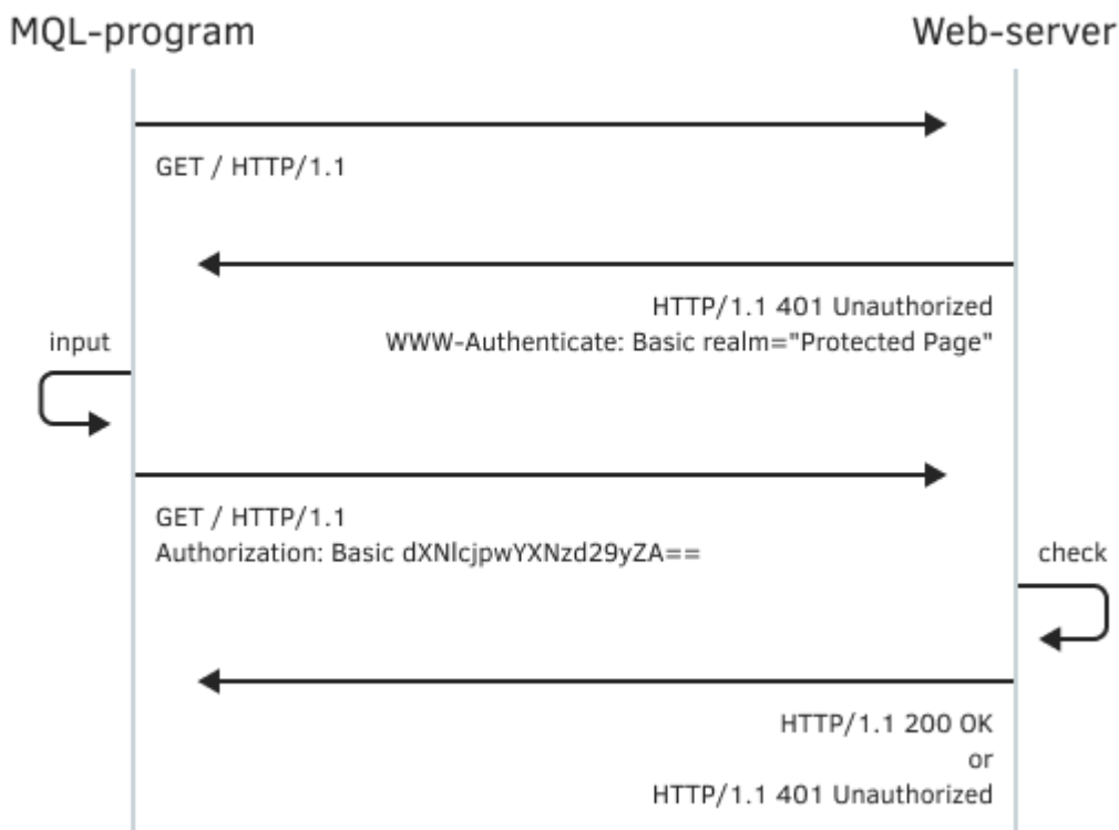
Simple authorization scheme on a web server
