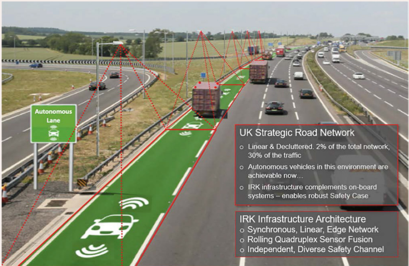
IRK proposes that its infrared-based autonomous technology could transform road travel, enabling lorries to move while their driver rests and taking tax and toll payments on the go
