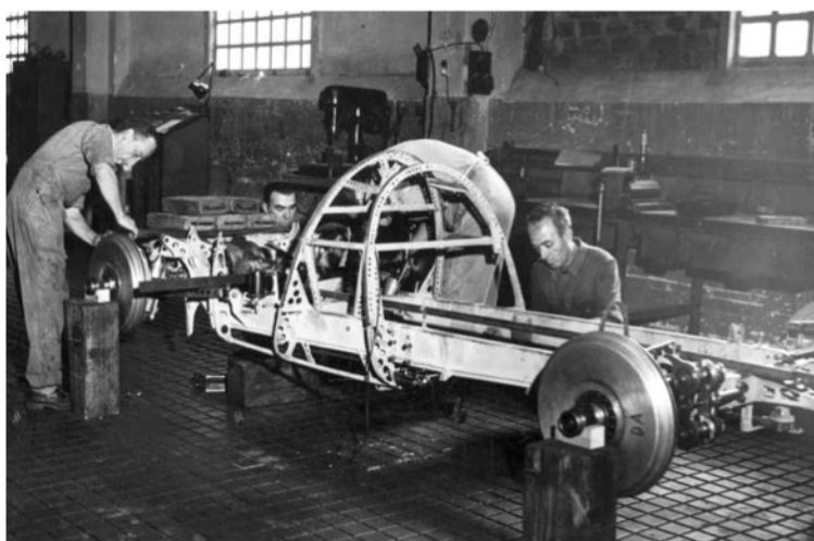
Following rule changes in 1938, Alfa engineers prepared a new chassis for its Types 312 and 316, carrying their suspension designs over from the 12C-37. Arches at the cowl held twin fuel tanks
