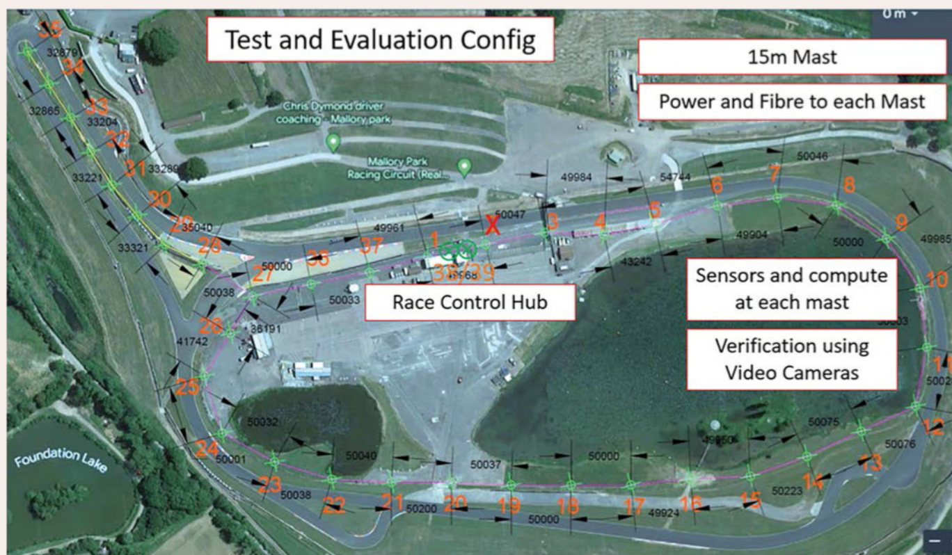
Plan of the IRK system demonstration at Mallory Park. The route featured 39 posts mounted with sensors and computers; any posts can be used, meaning any track can run the technology
