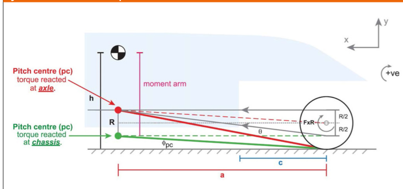
Fig 1: Force-based anti-dive and anti-squat
