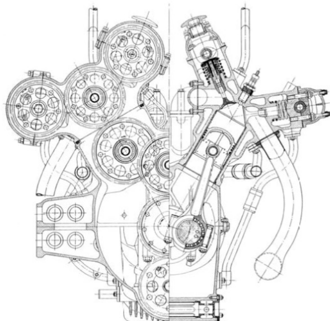
Seen in its 3.0-litre configuration for 1938 / '39, the Trevisan-designed Alfa V12 now had roller bearing big ends. The gear train for its cam drive was at the rear
