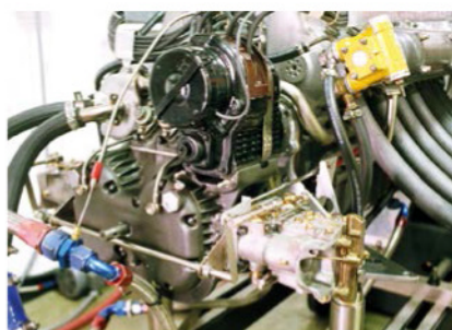
As installed in its post-war version, the Type 312 had the two Roots blowers visible side-by-side, sharing a single cover. Each was fed by its own carburettor
