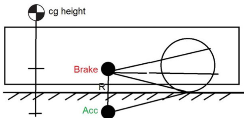
Fig 2: Poorly conditioned anti-dive and anti-squat
