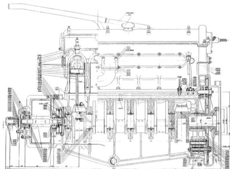
As configured for the Type 312, which arrived in time for the Tripoli Grand Prix in May 1936, the front gear train is now driving two Roots-style compressors, each serving one of the two banks of six cylinders
