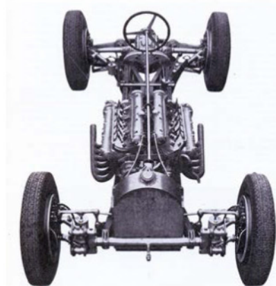
As rolled out for the 1937 season, the Type 12C-37 shows its very narrow central frame, a characteristic that did not serve it particularly well
