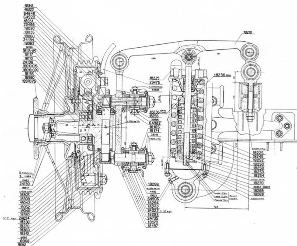
Used in both road and racecars by Alfa Romeo, this was the detail of the elaborate front suspension. Note the near vertical kingpins
