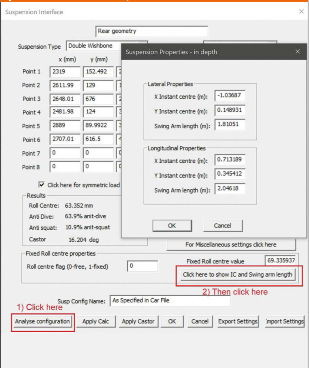
Fig 5: ChassisSim instant centre university
